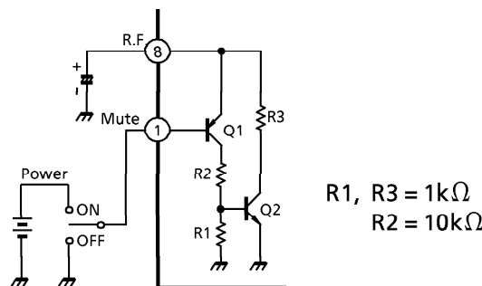
Fig. 4 Mute Circuit
